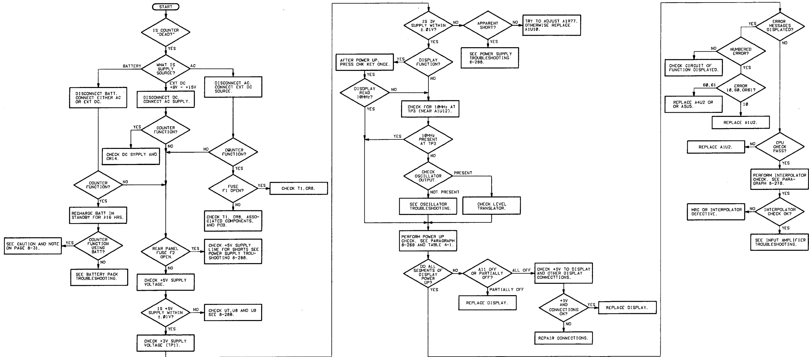
Figure 8-49. Troubleshooting Flowchart
