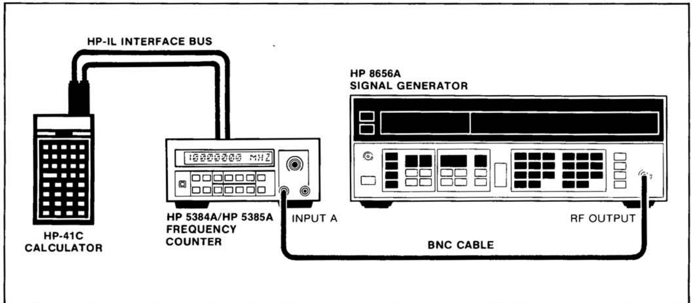
Figure 3-12. Example 5 Set-Up
